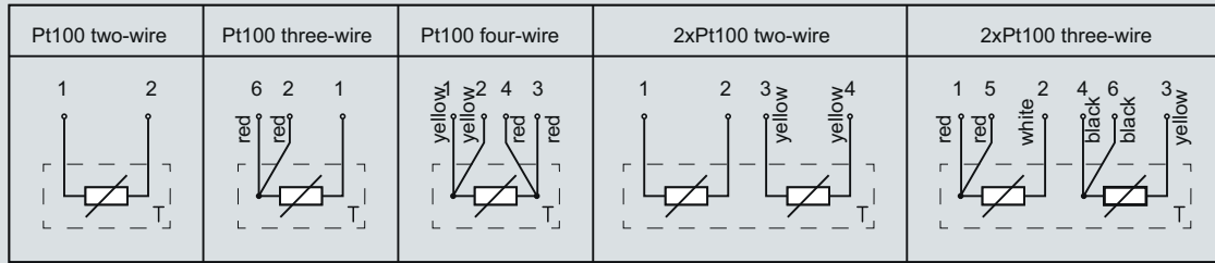
Connection diagram
