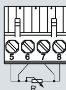
Four-wire system
