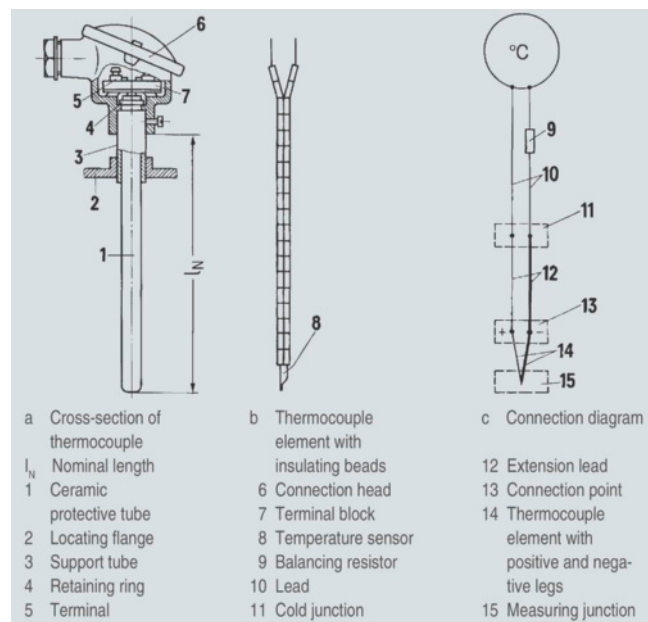
Thermocouple element
