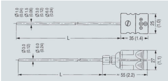
Jacket thermocouple with socket; at top with one thermocouple, at bottom with two thermocouples; dimensions in mm (inches)
