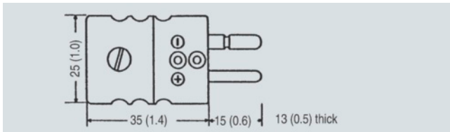
Coupling plug, dimensions in mm (inches)
