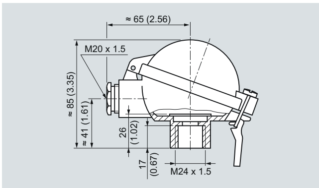
Connection head, form B, degree of protection IP65, made of cast light alloy, with standard hinged cover, dimensions in mm (inches)
