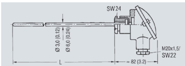
Jacket thermocouple with connection head, form B, made of cast light alloy, dimensions in mm (inches)
